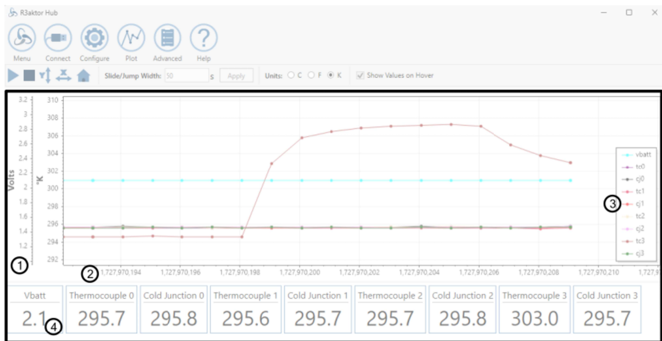
Figure 9: Plot layout
